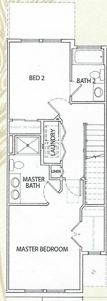
THIRD FLOOR
