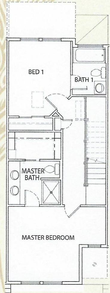
THIRD FLOOR
